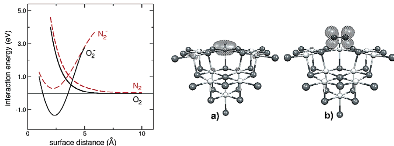
FIGURE 5. Spin-density plot for (a) (\text{H}^+)(\text{e}^-) centers located at a cationic reverse corner and (b) the complex formed by the interaction with \text{N}_2 or \text{O}_2 molecules. On the left-hand side, the schematic potential energy curves for the interaction of \text{O}_2 (solid curve) and \text{N}_2 (red dotted curve) molecules is shown. Negative values indicate bound states.
